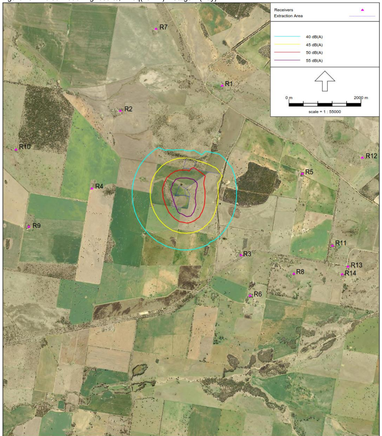
Figure 18 – Noise modelling results, LAeq(15min) – Stage 1 (Day)
